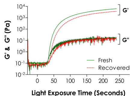
Figure 5. Evolution of elastic ( G' ) and viscous ( G'' ) moduli during in situ gelation of PEG4NB-DTT using fresh or recovered eosin-Y at 0.1 mM as photoinitiator (PEG4NB: 10 wt %, N = 3 ). Error bars were neglected for clarity.
