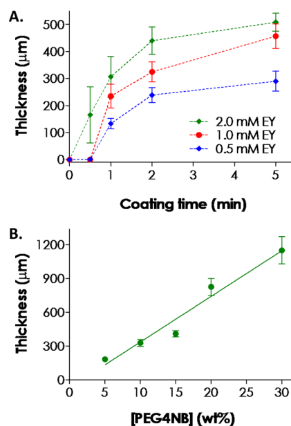
Figure 7. (A) Effect of secondary visible-light exposure time (or coating time) and eosin-Y concentration in the core gel on the thickness of thiol-ene hydrogel coating. (B) Effect of PEG4NB macromer concentration on the thickness of thiol-ene hydrogel coating (eosin-Y in the core gel: 2.0 mM; coating time: 2 min). Core gels were fabricated with 10 wt % PEG4NB. ( N = 3 ; mean \pm S.D.)
