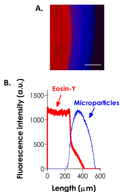
Figure 6. (A) Fluorescence micrograph and (B) intensity profile of a dual-layer hydrogel formed by sequential visible-light-mediated thiol-ene photopolymerization. Red and blue fluorescence were from the eosin-Y added in the core gel and blue microparticles added in the coating macromer solution, respectively. (Conditions: 10 wt % PEG4NB-DTT preformed gel with 2.0 mM eosin-Y, 10 wt % PEG4NB-DTT and 2 min of secondary polymerization, 5% blue particles; scale bar = 200 \mu\text{m} .)
