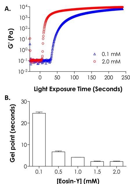
Figure 1. Effect of eosin-Y concentration on (A) gelation kinetics and (B) gel points of PEG4NB-DTT hydrogels formed by visible-light-mediated thiol-ene photopolymerization. (PEG4NB: 10 wt %; N = 3 ; mean \pm standard deviation (S.D.).)
